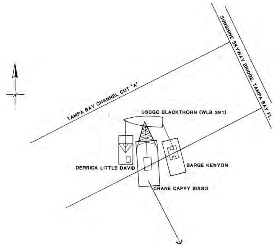
Lifting arrangements for Blackthorn .
