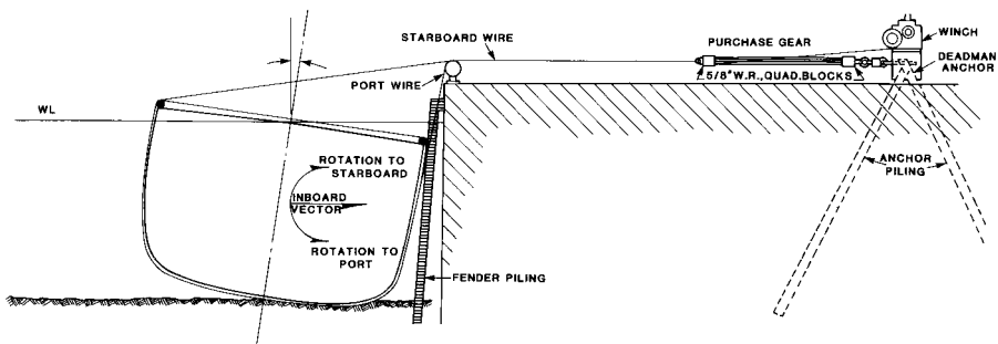
This rigging was used to keep Oriental Warrior upright.
