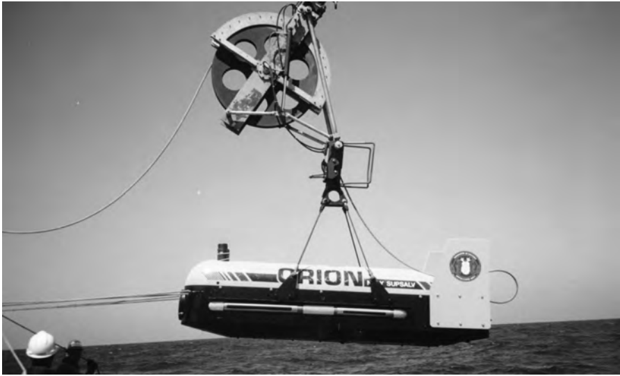
ORION side-scan sonar system.
