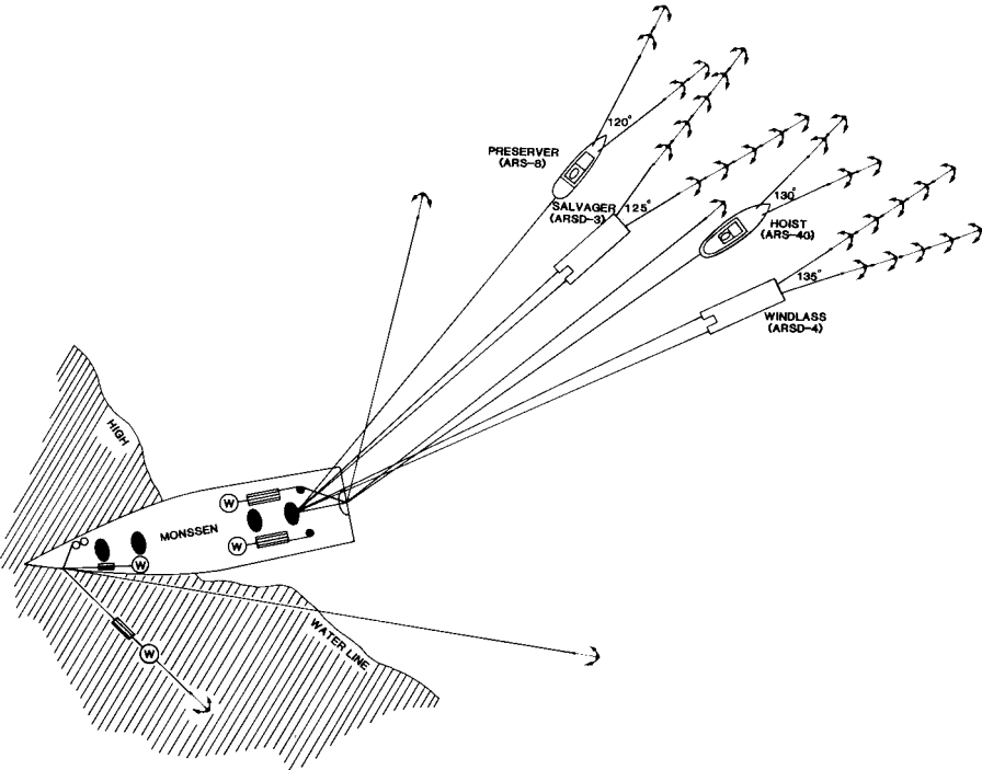
These pulling arrangements freed Monssen .
